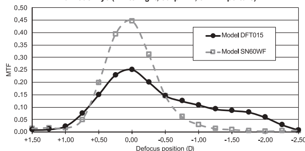
Figure 4: Modulation Transfer Function (MTF) Through-Focus Response of 20.0 D IOLs in a Model Eye (White Light, 50 lp/mm, 3 mm Aperture)
