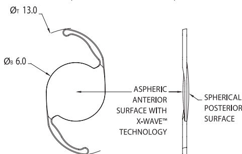
Figure 2: Physical Characteristics of AcrySof™ IQ Vivity™ Toric IOLs (All dimensions in millimeters)
