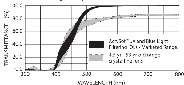
Figure 3: Spectral Transmittance
